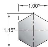
Zinc Anode Schematic
