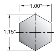
Zinc Anode Schematic
