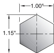
Zinc Anode Schematic
